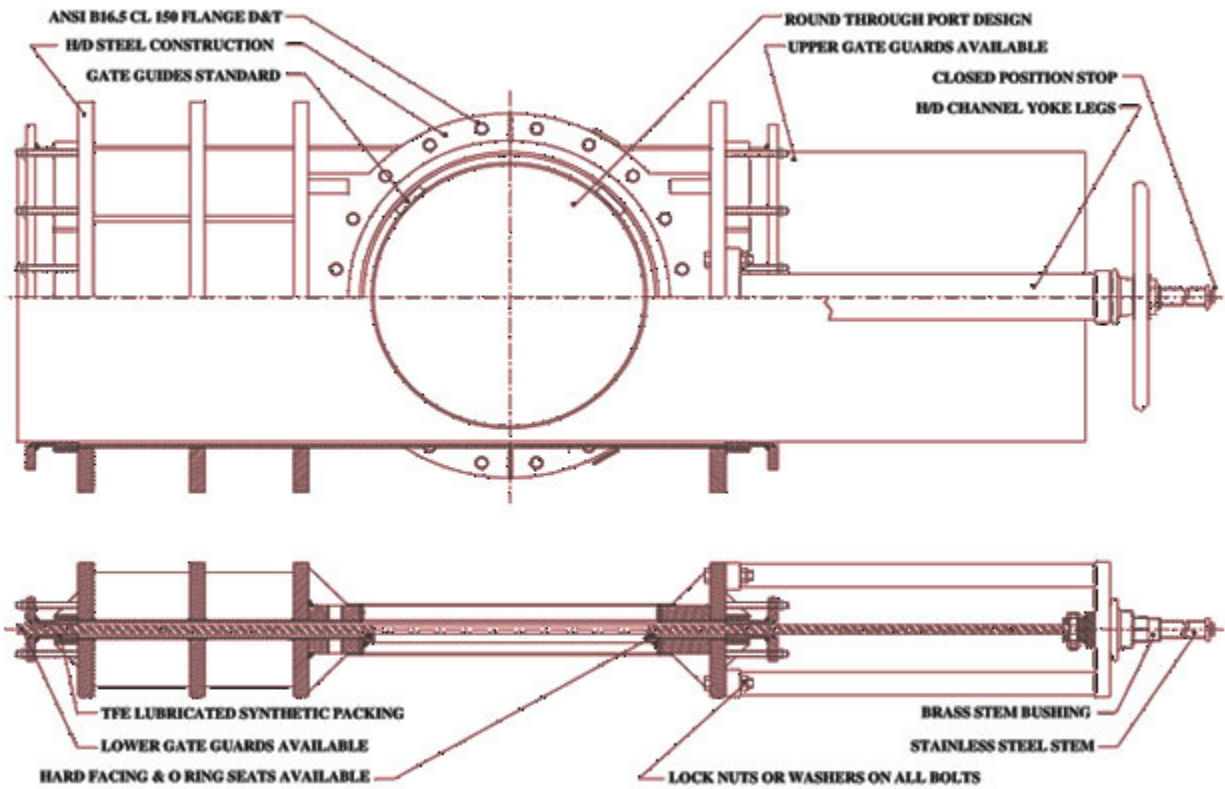
VALVE SHOWN IN OPEN POSITION
