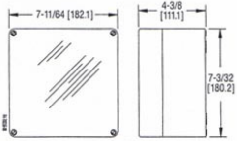
4 MOUNTING LOCATIONS CENTERED 4-23/32 [120] APART ON BACK OF ENCLOSURE
