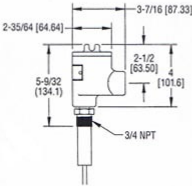
4 MOUNTING LOCATIONS CENTERED 4-23/32 [120] APART ON BACK OF ENCLOSURE
